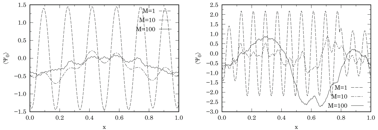
Fig. 1 We show the ground state from Eq. (3.2) for three choices of increasing M and N = 3, L = 1 . Low g = 1 in the left panel and high g = 100 in the right panel. From Eq. (3.3) the resulting ground state energy is as follows: for g = 1 \rightarrow (\tilde{E}_0 = 741.956 for M = 1 , \tilde{E}_0 = 148.428 for M = 10 , and \tilde{E}_0 = 613.504 for M = 100 ) and for g = 100 \rightarrow (\tilde{E}_0 = 3027.62 for M = 1 , \tilde{E}_0 = 2343.16 for M = 10 , and \tilde{E}_0 = 3698.51 for M = 100 )
