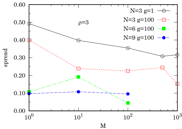
Fig. 2 We show the ground state wavefunction spread of Eq. (3.4) as a function of the Monte Carlo steps M for m = 1, \rho = 3 and the four cases N = 3, L = 1, g = 1 , N = 3, L = 1, g = 100 , N = 6, L = 2, g = 100 , and N = 9, L = 3, g = 100
