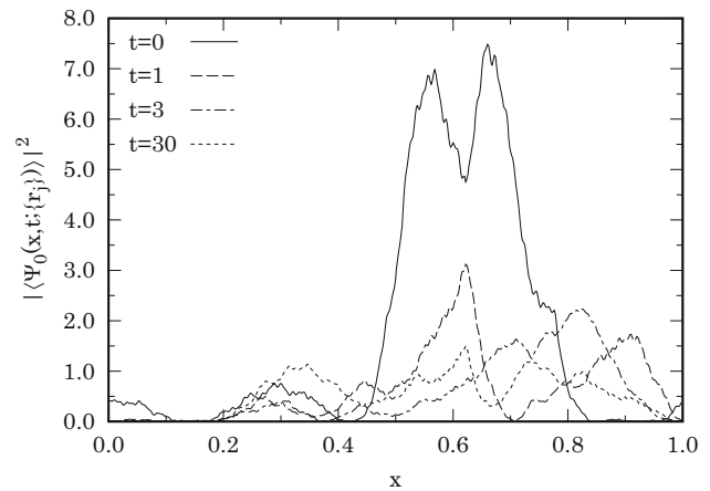
Fig. 3 We show the time evolution of |\tilde{\Psi}_0(x, t)|^2 from Eq. (3.8) for N = 3, L = 1, g = 100, M = 100 at t = 0, 1, 3, 30
